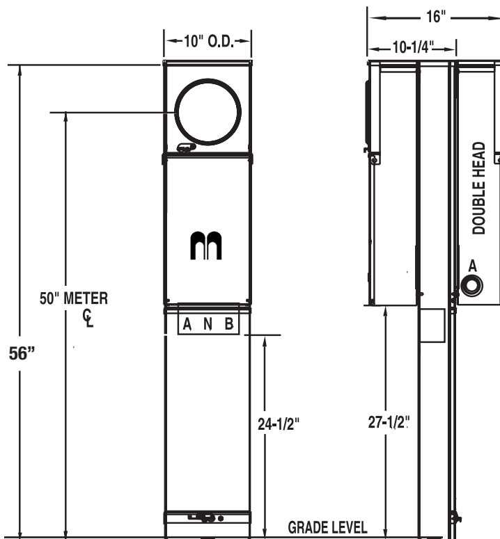
Series wired main shown with optional K5400-520GR kit
