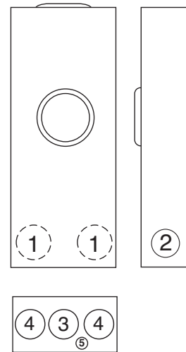
200 AMP-4 TERMINAL-METER MAIN WITH BREAKERS-1Ø3W-RINGLESS-120 / 240 VAC
